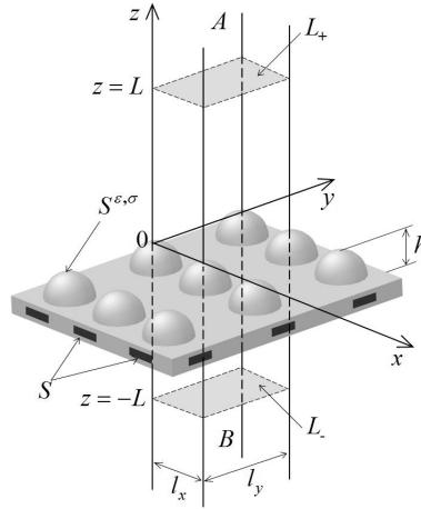
Figure 1. Geometry of a two-dimensionally periodic grating.
