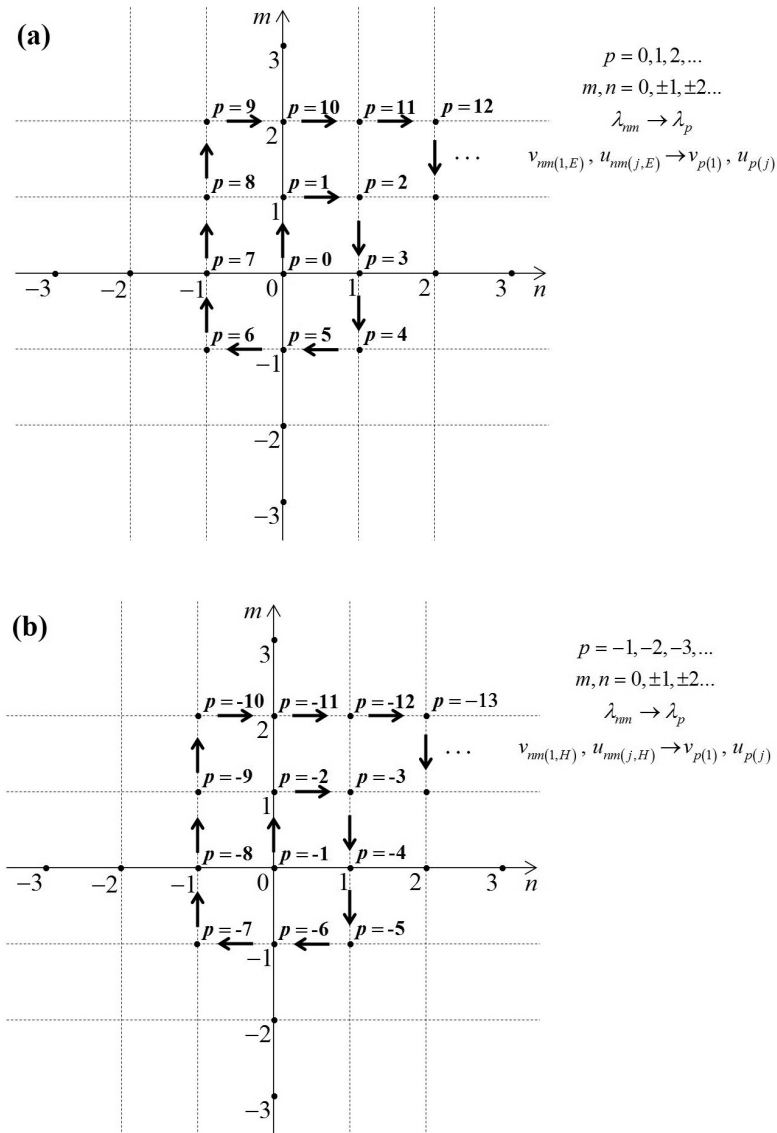
Figure 3. Construction of sets of the values v_{p(1)} , u_{p(j)} , and \lambda_p ( p = 0, \pm 1, \pm 2, \dots ) from sets of the values v_{nm(1,E)} , u_{nm(j,E)} , v_{nm(1,H)} , u_{nm(j,H)} , and \lambda_{nm} ( m, n = 0, \pm 1, \pm 2, \dots ): (a) p = 0, 1, 2, \dots ; (b) p = -1, -2, -3, \dots
